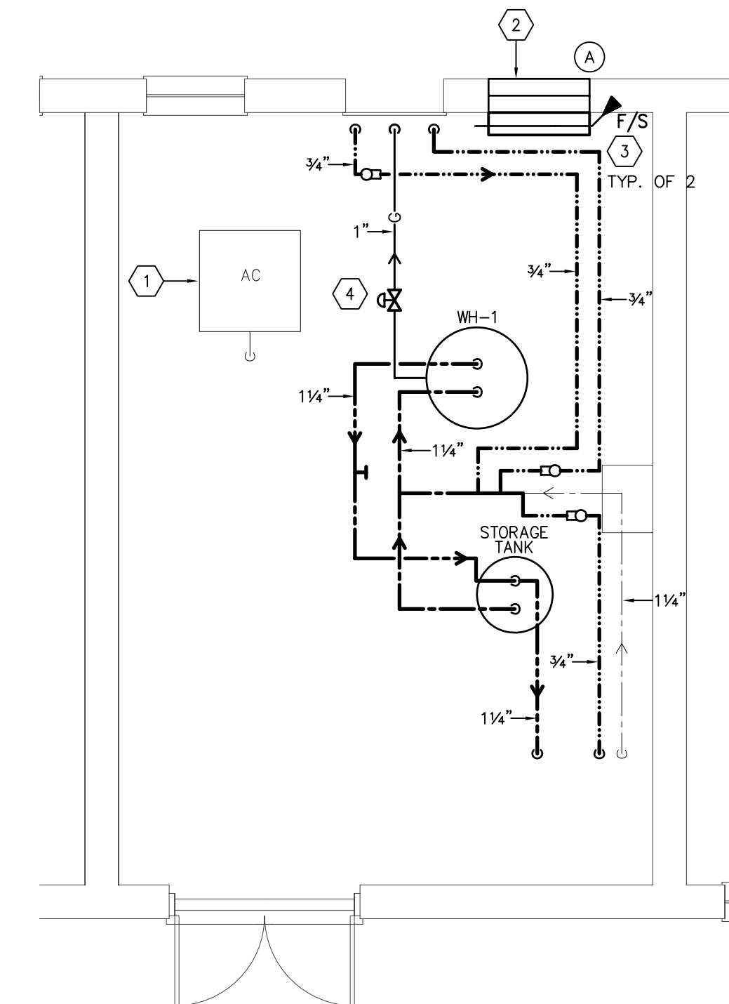
1 ENLARGED PLAN RM. 202 P2.2 SCALE: 1/4" = 1'-0"
